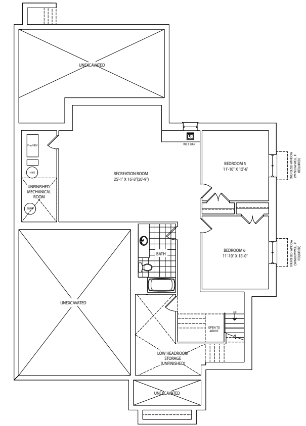
BASEMENT PLAN ELEVATION A
