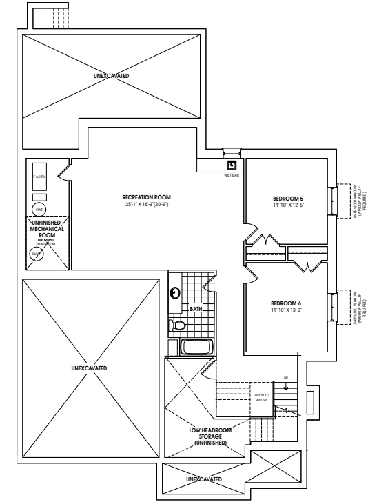
BASEMENT PLAN ELEVATION C
