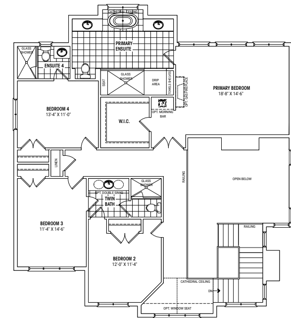
SECOND FLOOR PLAN ELEVATION C
