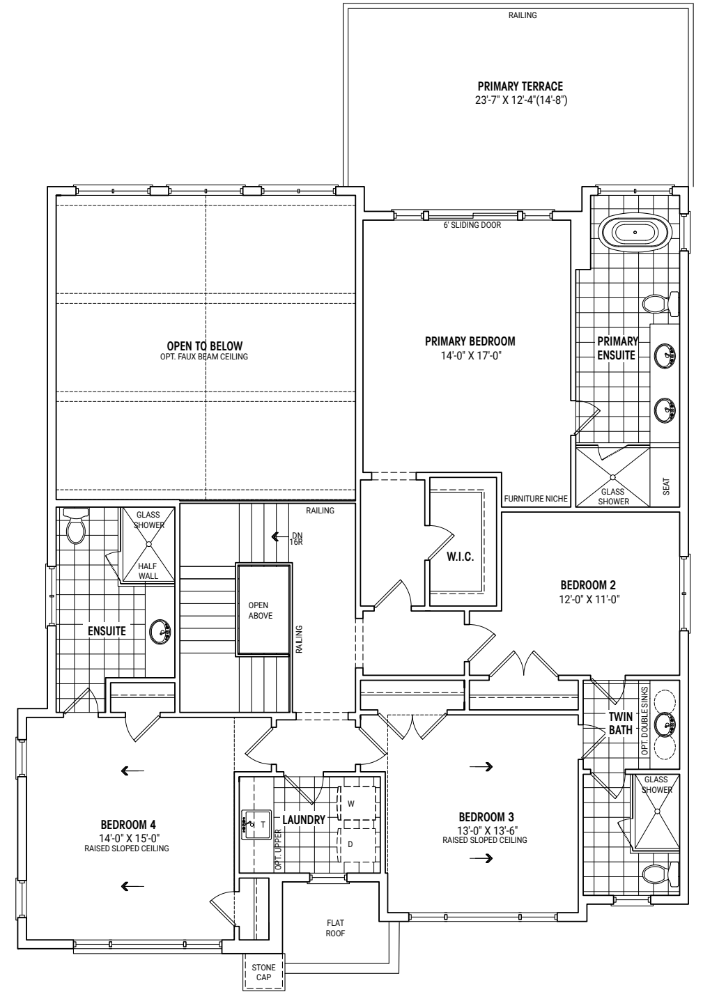
SECOND FLOOR PLAN ELEVATION B
