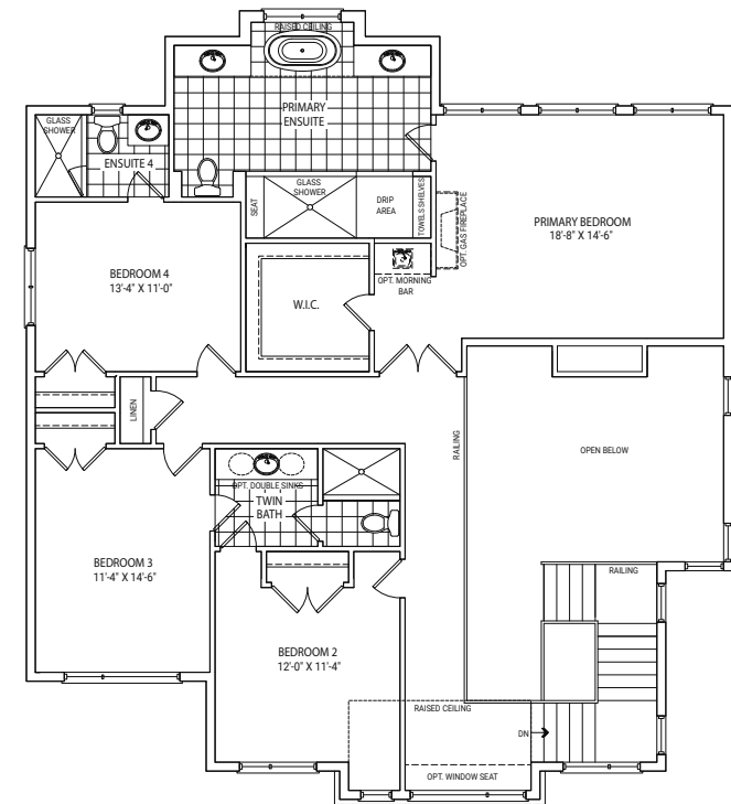
SECOND FLOOR PLAN ELEVATION A
