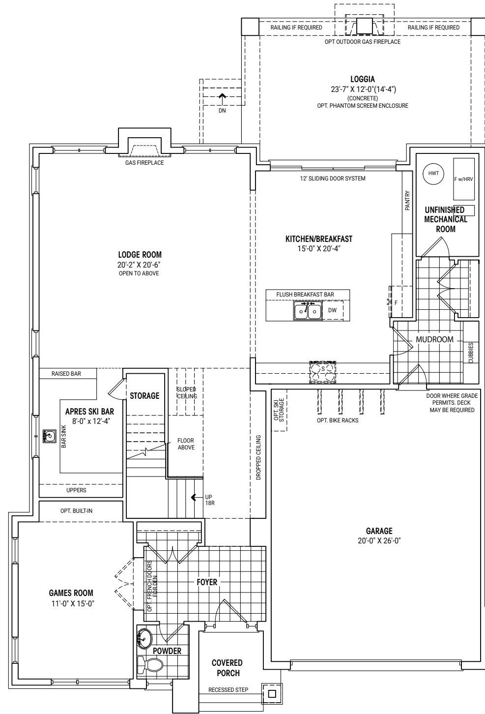
GROUND FLOOR PLAN ELEVATION B
